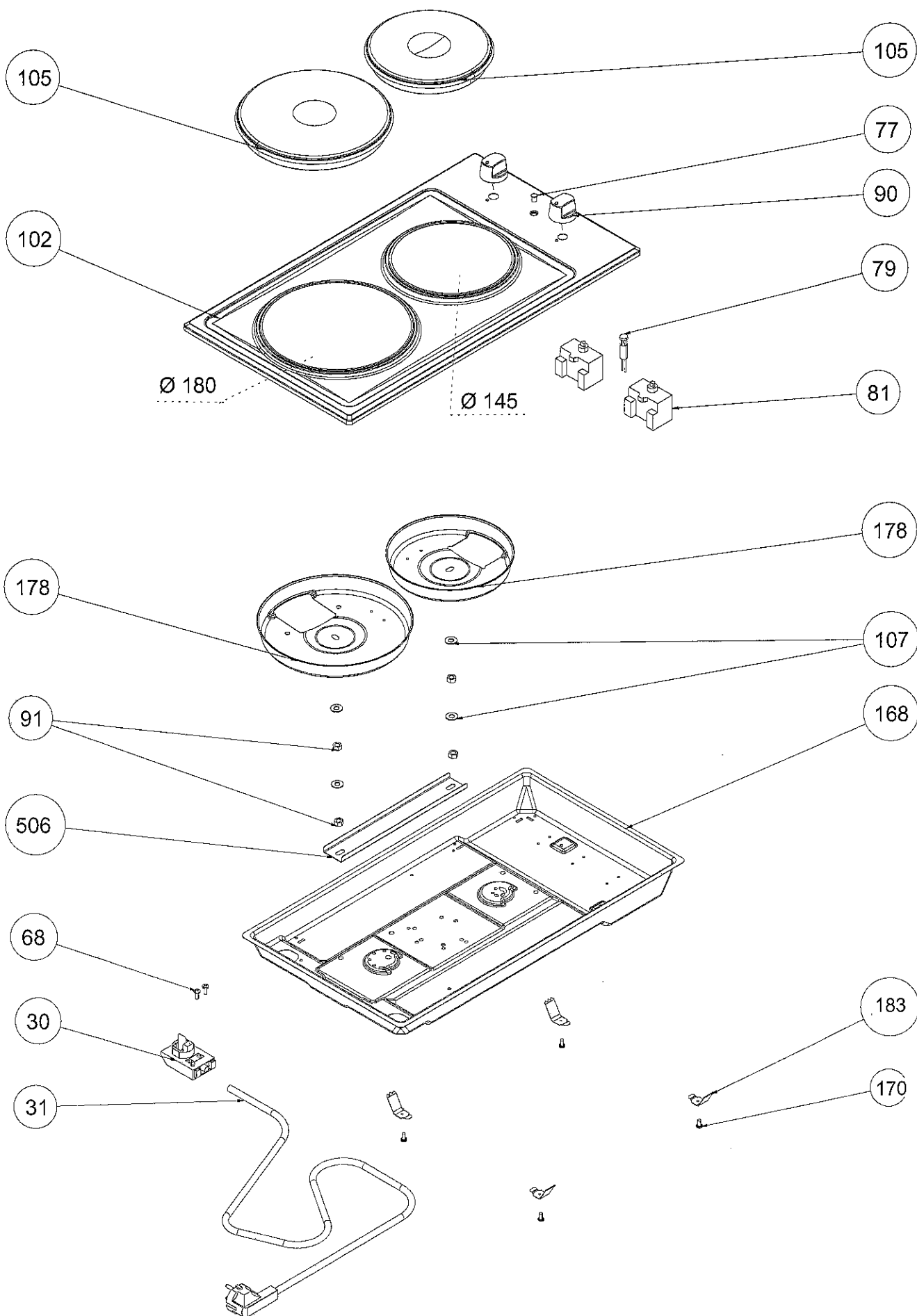
EXPLODED VIEW - DOMINO 2 ELC HOB ASSEMBLY
